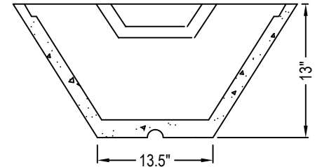
FRONT SECTION
