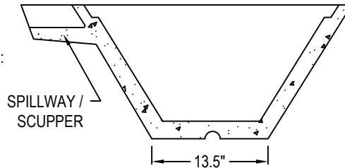
SIDE SECTION
